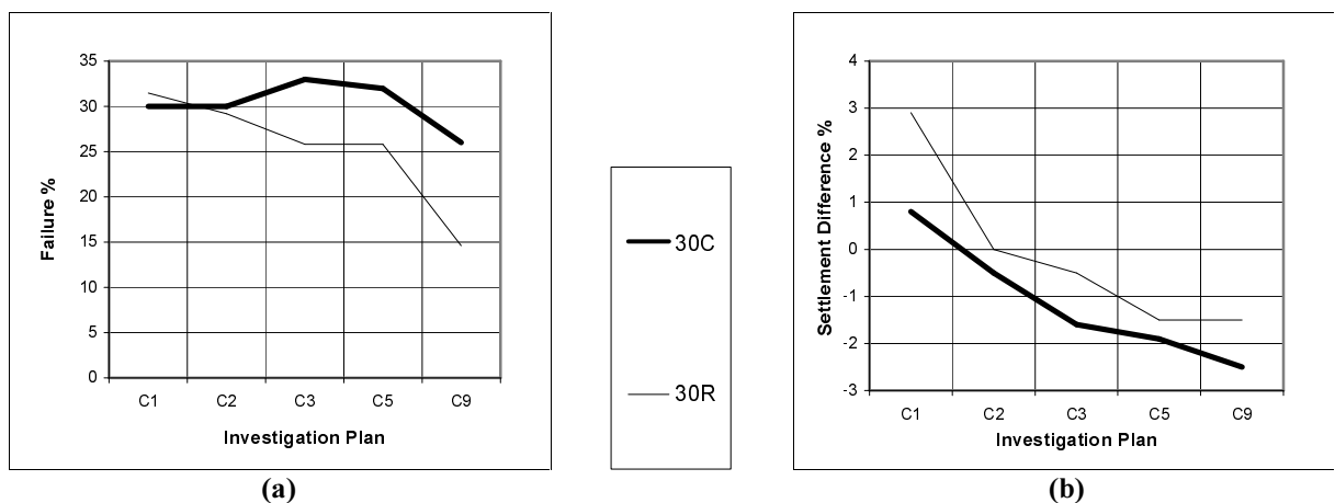
Figure 7. (a) Failure Probability from Schmertmann's Method and (b) Settlement Difference from Finite Element Method Each Using Site Investigation Data and Complete Knowledge.
