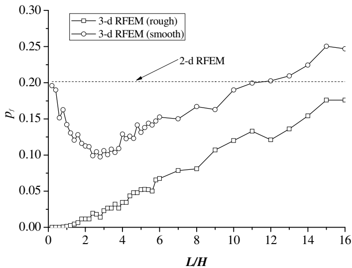
Fig. 12. Probability of failure versus slope length ratio ( V_{c_u} = 0.5 , \theta = H , FS = 1.39 , slope angle 2h : 1v)
