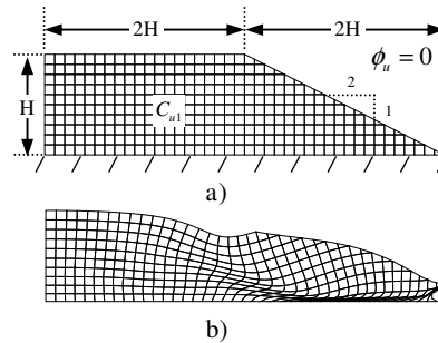
Fig. 7. Undrained slope without foundation
