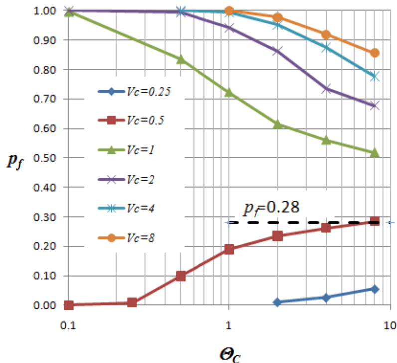
Fig. 3. Influence of the spatial correlation length and coefficient of variation on the probability of failure of an undrained slope ( \mu_C = 0.25 ).
