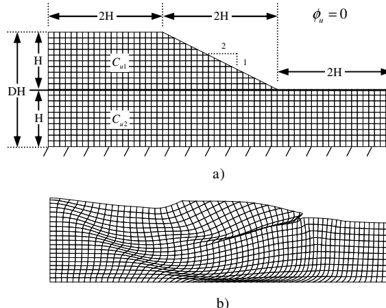
Fig. 8. Undrained two-layer slope
