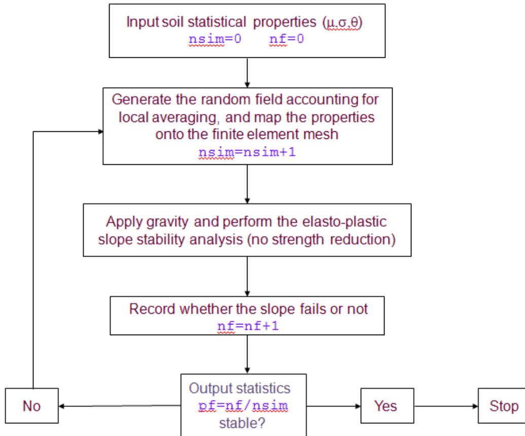
Fig. 1. Flow chart for a typical RFEM slope stability analysis.
