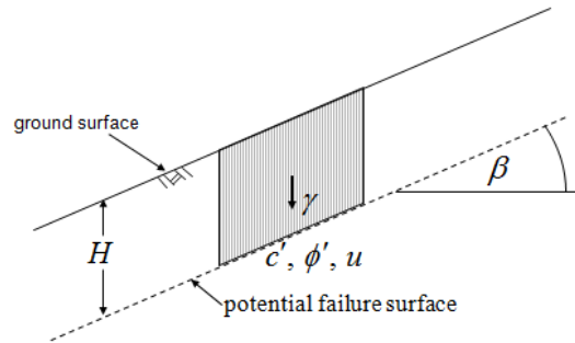
Fig. 5. Geometry and parameters of an infinite slope
