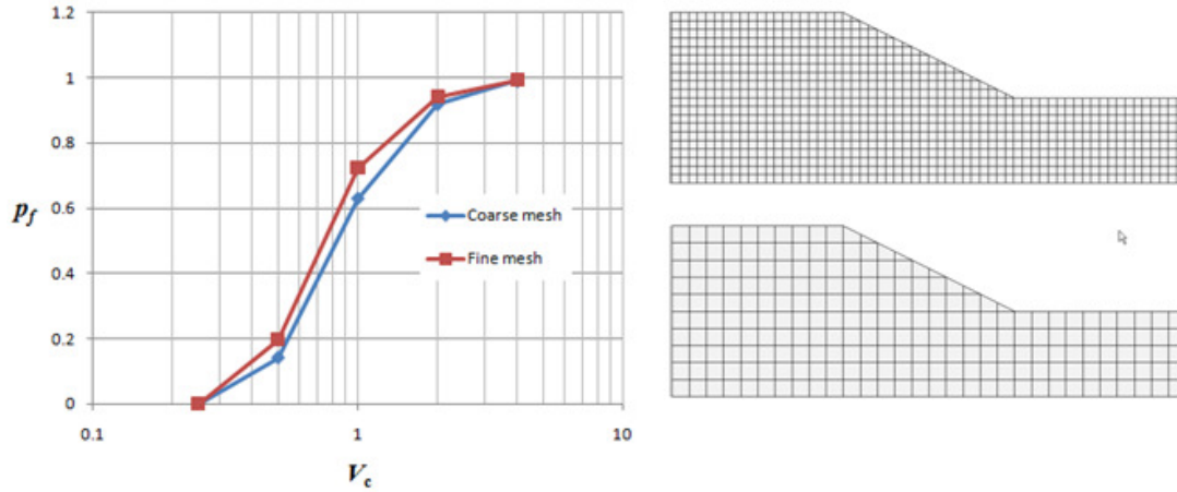
Fig. 4. Influence of mesh density on p_f for an undrained slope with \Theta_c = 1 and \mu_c = 0.25
