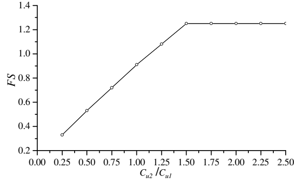
Fig. 9. Influence of C_{u2} / C_{u1} on the FS of the two-layer slope in Fig. 8
