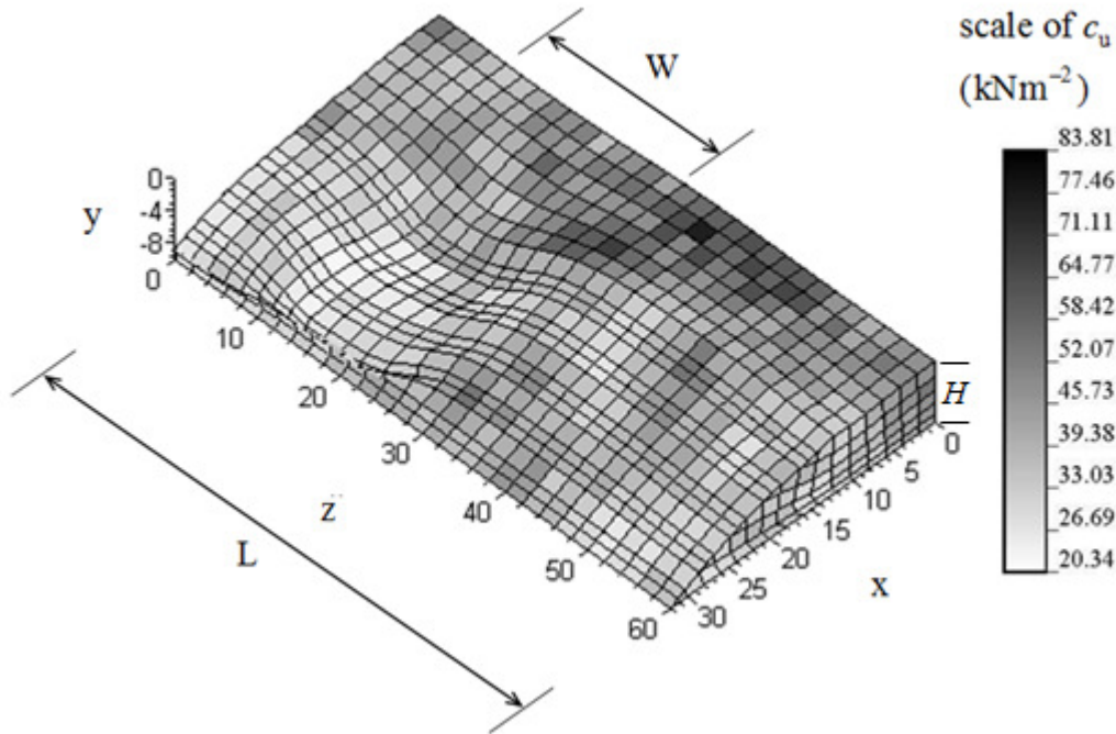
Fig. 11. Slope failure with \theta = 2H (isotropic) and rough boundary condition
