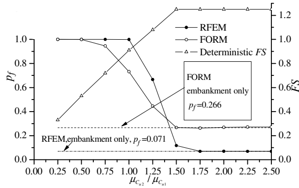
Fig. 10. Influence of \mu_{C_{u2}} / \mu_{C_{u1}} on the p_f of undrained slopes by RFEM ( \mu_{C_{u1}} = 0.153 , v_{C_{u1}} = v_{C_{u2}} = 0.3 and \Theta_{\ln C_{u1}} = \Theta_{\ln C_{u2}} = 0.5 ).
