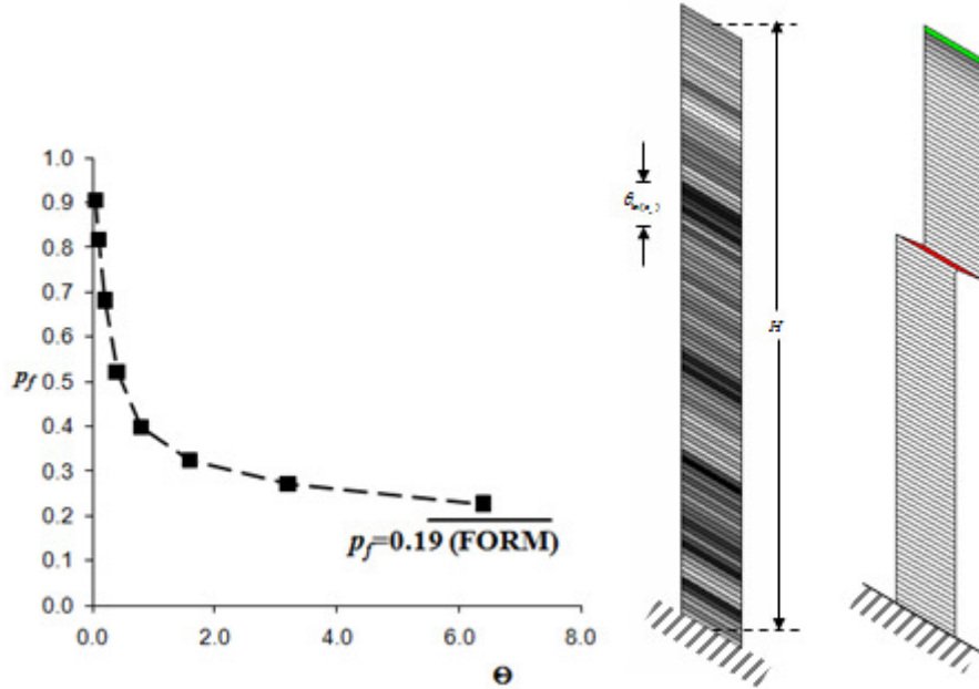
Fig. 6. Comparison of RFEM and FORM results for an infinite slope analysis.
