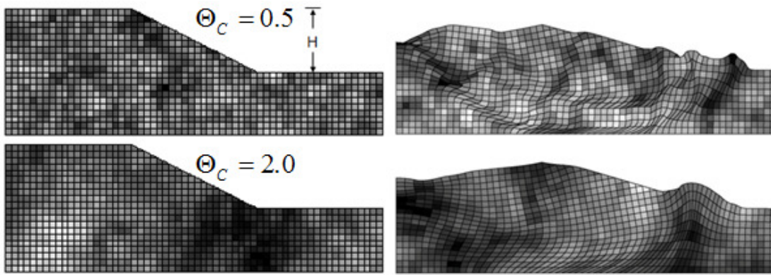
Fig. 2. Typical failure mechanisms from an RFEM analysis with two different spatial correlation lengths.
