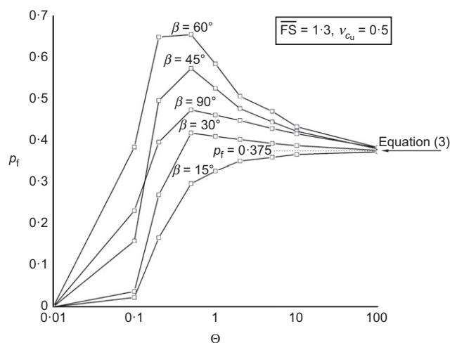
Fig. 5. Probability of failure plotted against dimensionless spatial correlation length with different slope angles
