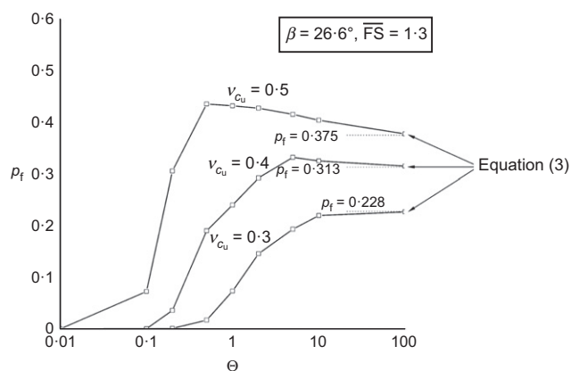
Fig. 4. Probability of failure plotted against dimensionless spatial correlation length with different coefficients of variation
